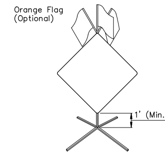
PORTABLE/TEMPORARY SIGN MOUNTING
