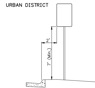
SIGN MOUNTING LOCATIONS
