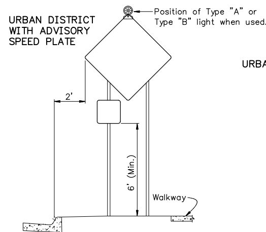
SIGN MOUNTING LOCATIONS
