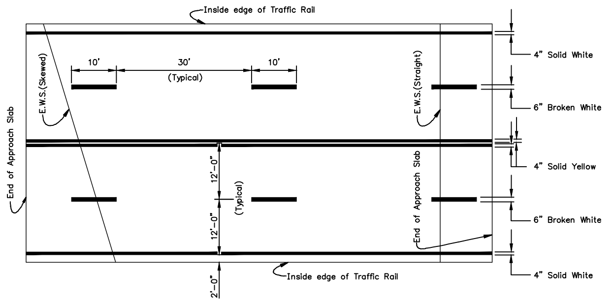
FOUR-LANE BRIDGE
