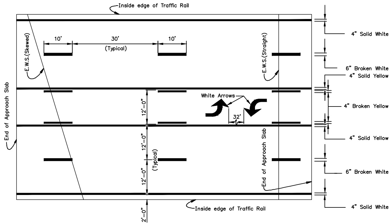
FIVE-LANE BRIDGE
