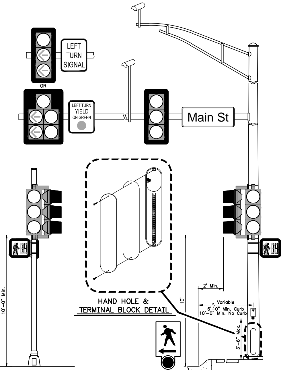
SIGNAL PEDESTAL
