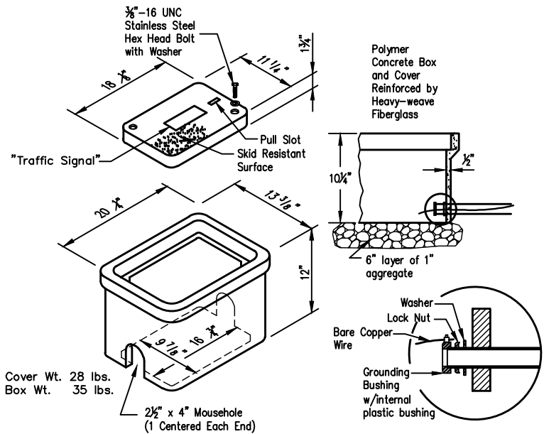
JUNCTION BOX DETAIL
