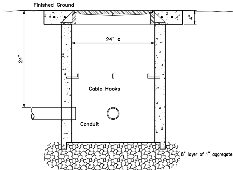
SERVICE BOX DETAIL
