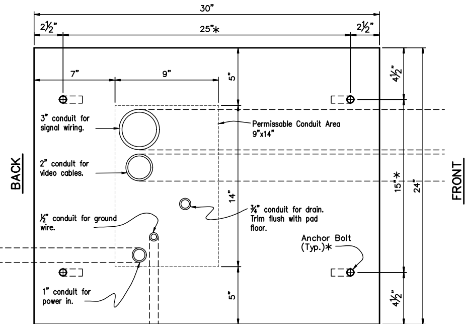
PAD DETAIL
