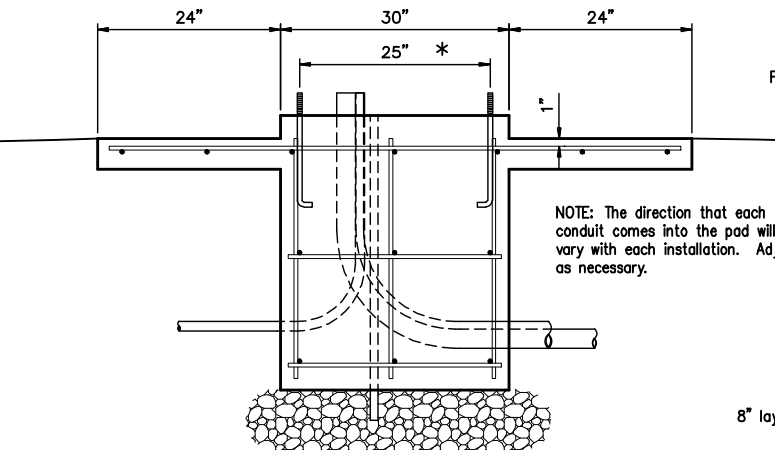
LEFT VIEW
