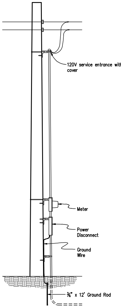
POWER SERVICE DETAIL
