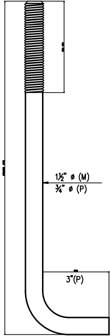
ANCHOR BOLT DETAILS
