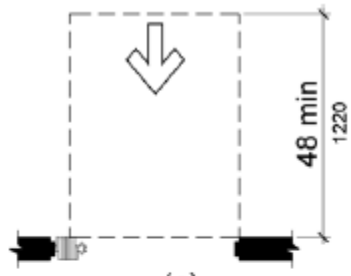
(a) front approach
