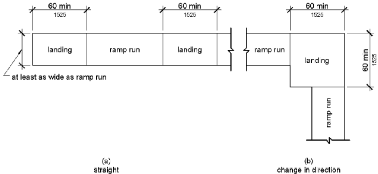
Figure 405.7 Ramp Landings
