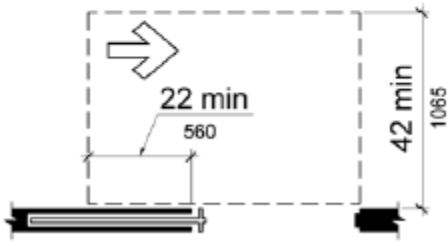
(c) pocket or hinge approach
