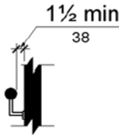
Figure 505.5 Handrail Clearance
