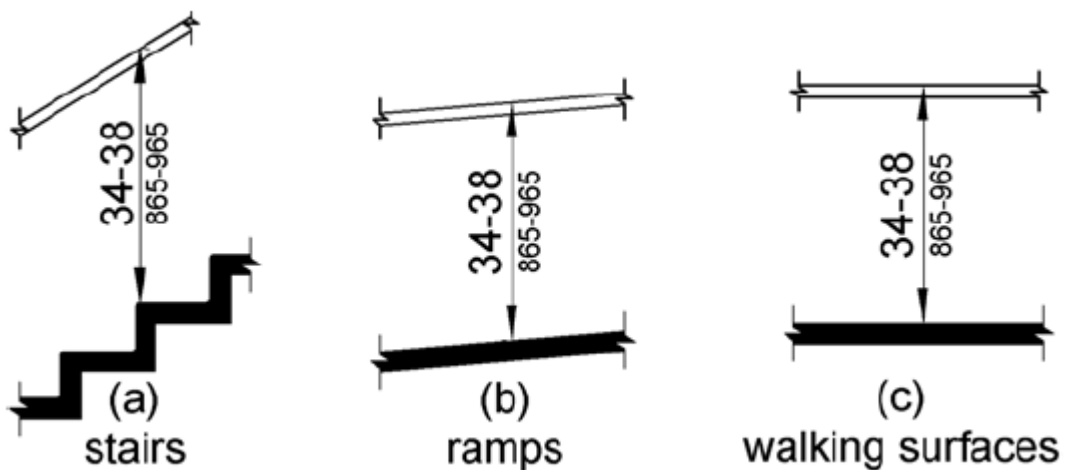
Figure 505.4 Handrail Height
