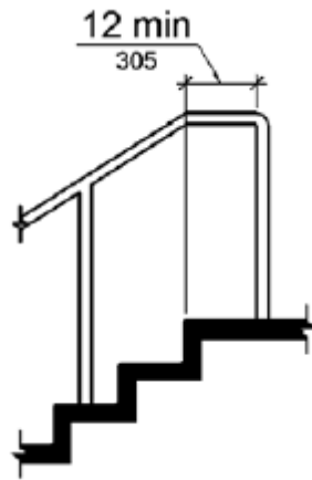
Figure 505.10.2 Top Handrail Extension at Stairs
