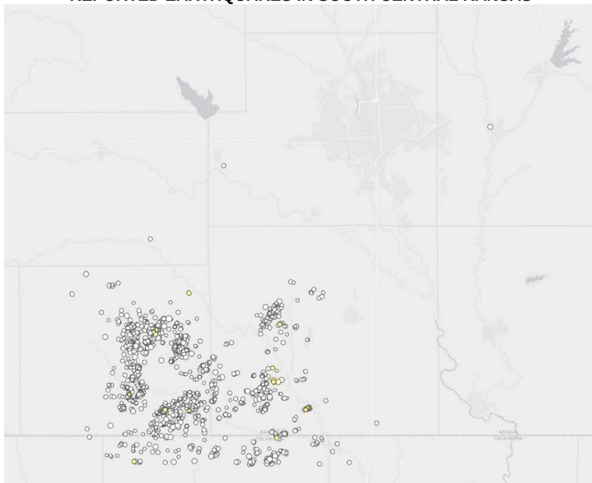
REPORTED EARTHQUAKES IN SOUTH CENTRAL KANSAS
