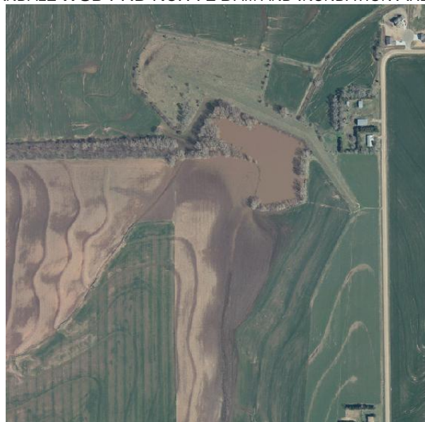
ANDALE WSD FRD NO. A-2 DAM AND INUNDATION AREA
