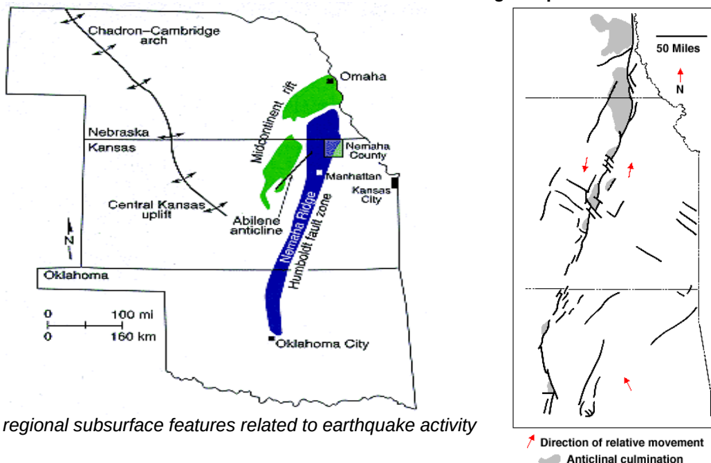
Humboldt Fault Zone / Nemaha Ridge Maps
