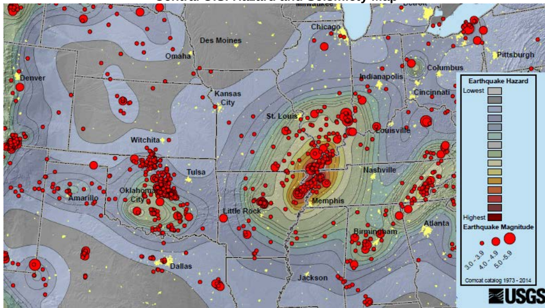
Central U.S. Hazard and Seismicity Map
