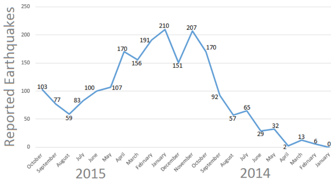
NUMBER OF REPORTED EARTHQUAKES PER MONTH FOR 2014 AND 2015
