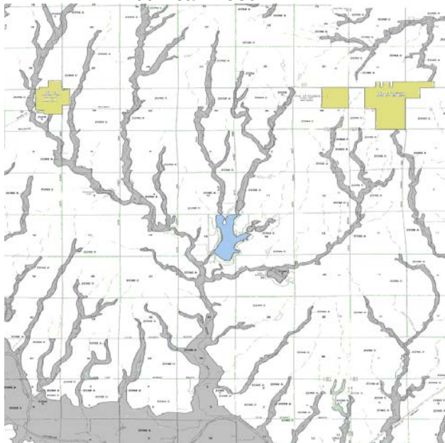
Lake Afton Flood Inundation Map 100-Year Flood
