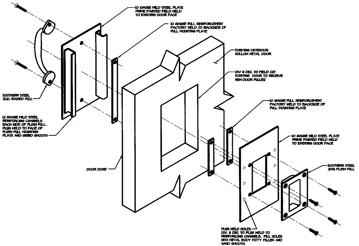
15 DOOR PULL RETRO-FIT (TYPICAL) DE8.0 SCALE: NONE
