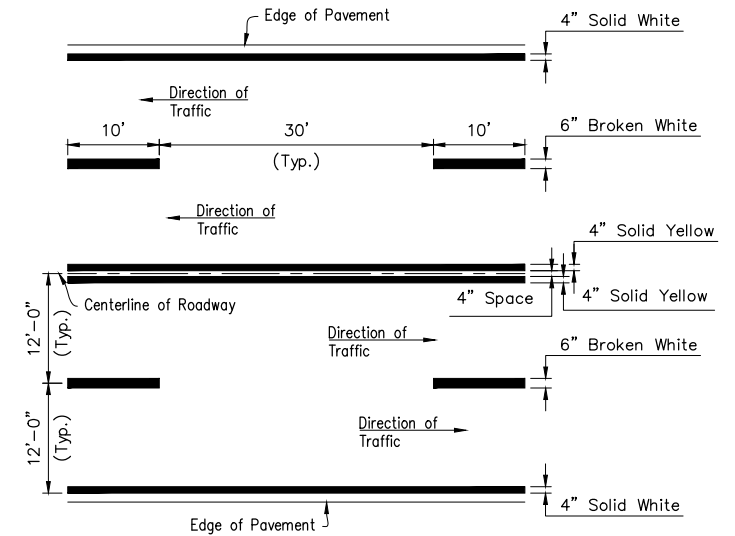
FOUR-LANE ROADWAY
