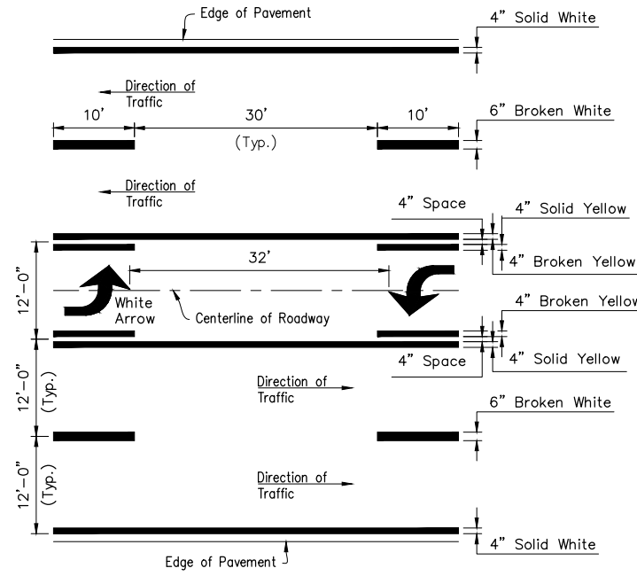
FIVE-LANE ROADWAY
