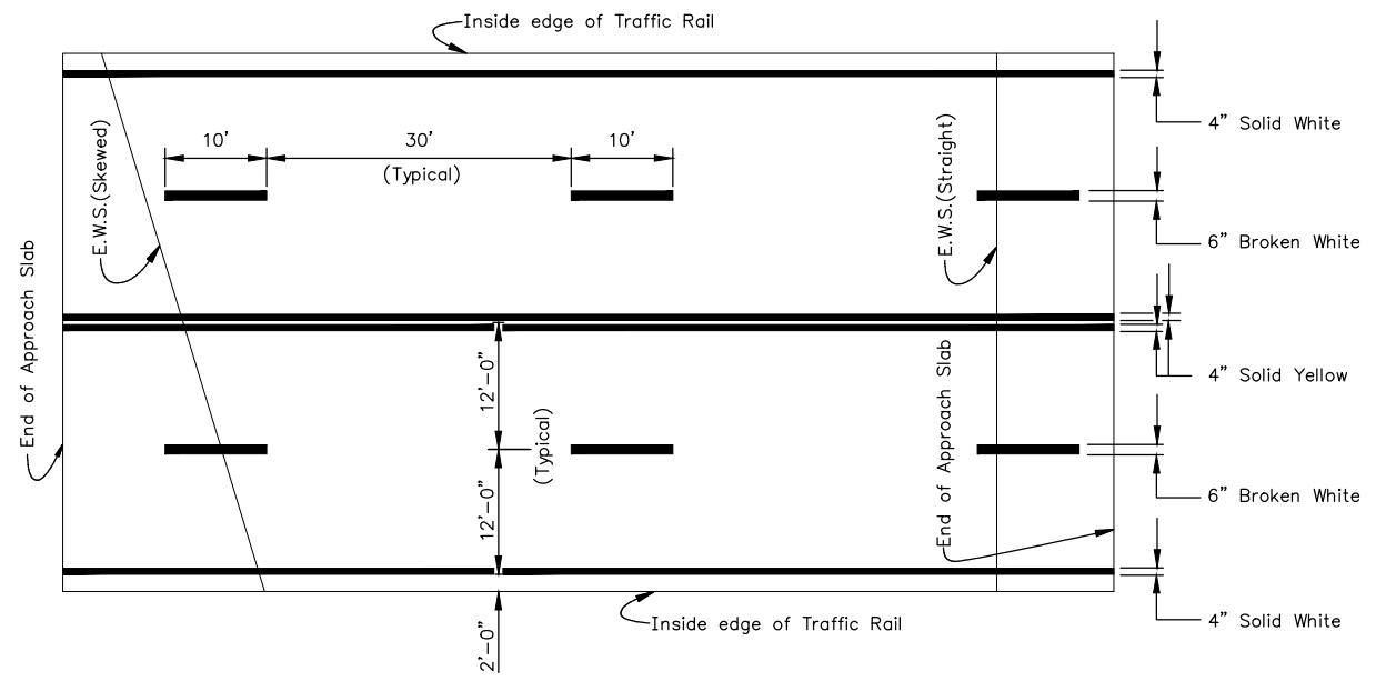
FOUR-LANE BRIDGE
