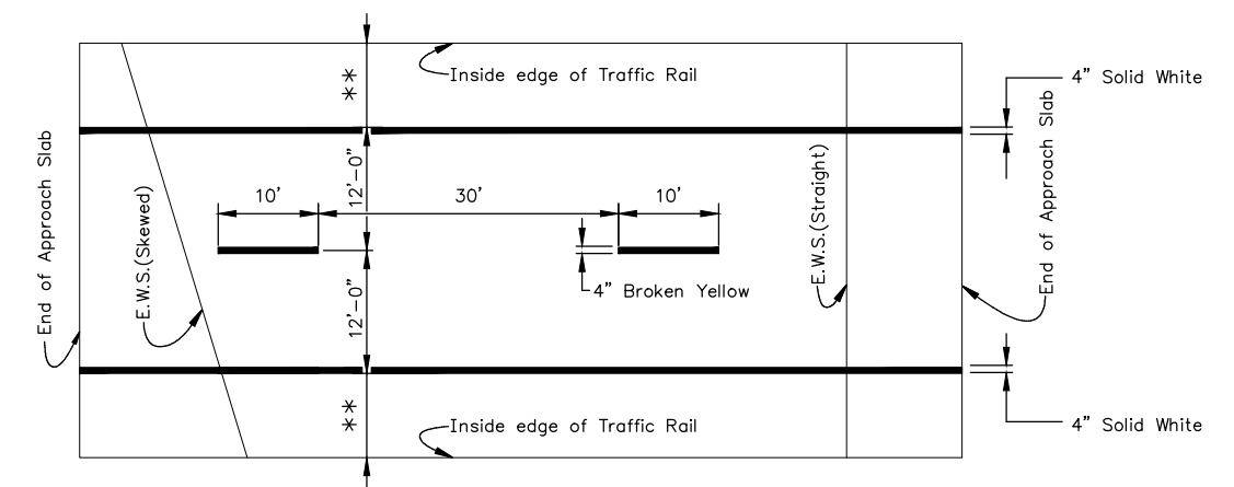
CENTERLINE (PASSING ALLOWED) (Bridge width greater than or equal to roadway approach width) ** Greater than or equal to approaching shoulder width.
