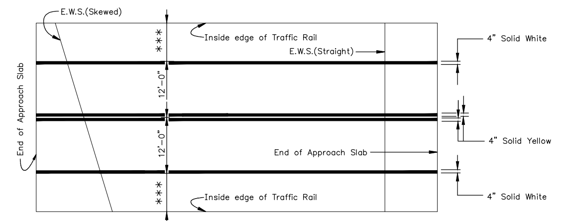
NO PASSING (TWO DIRECTIONS) (Bridge width less than roadway approach width) *** Less than approaching shoulder width.
