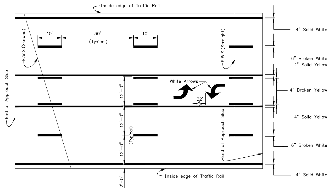
FIVE-LANE BRIDGE
